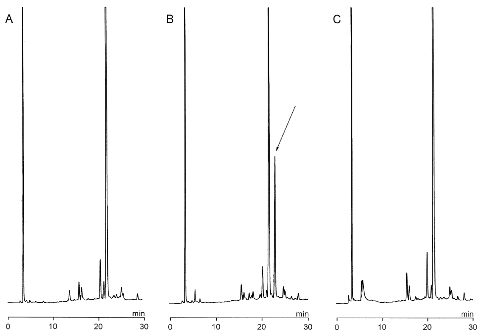
Figure 5 HPLC chromatograms of the crude peptide TGF z (34–43). Synthesis was performed using the derivatives Fmoc-His(1-Trt)-OH (A) or Fmoc-His(3-Bum)-OH (B) and final cleavage was carried out with cocktail B. The thiazolidine-derivative generated during cleavage of the Bum group is indicated by an arrow in chromatogram B. Crude TGF z (34–43) was also obtained by synthesis with the derivative Fmoc-His(3-Bum)-OH and final cleavage with cocktail D containing methoxyamine (C). Additional experimental details are given in Materials and Methods.
